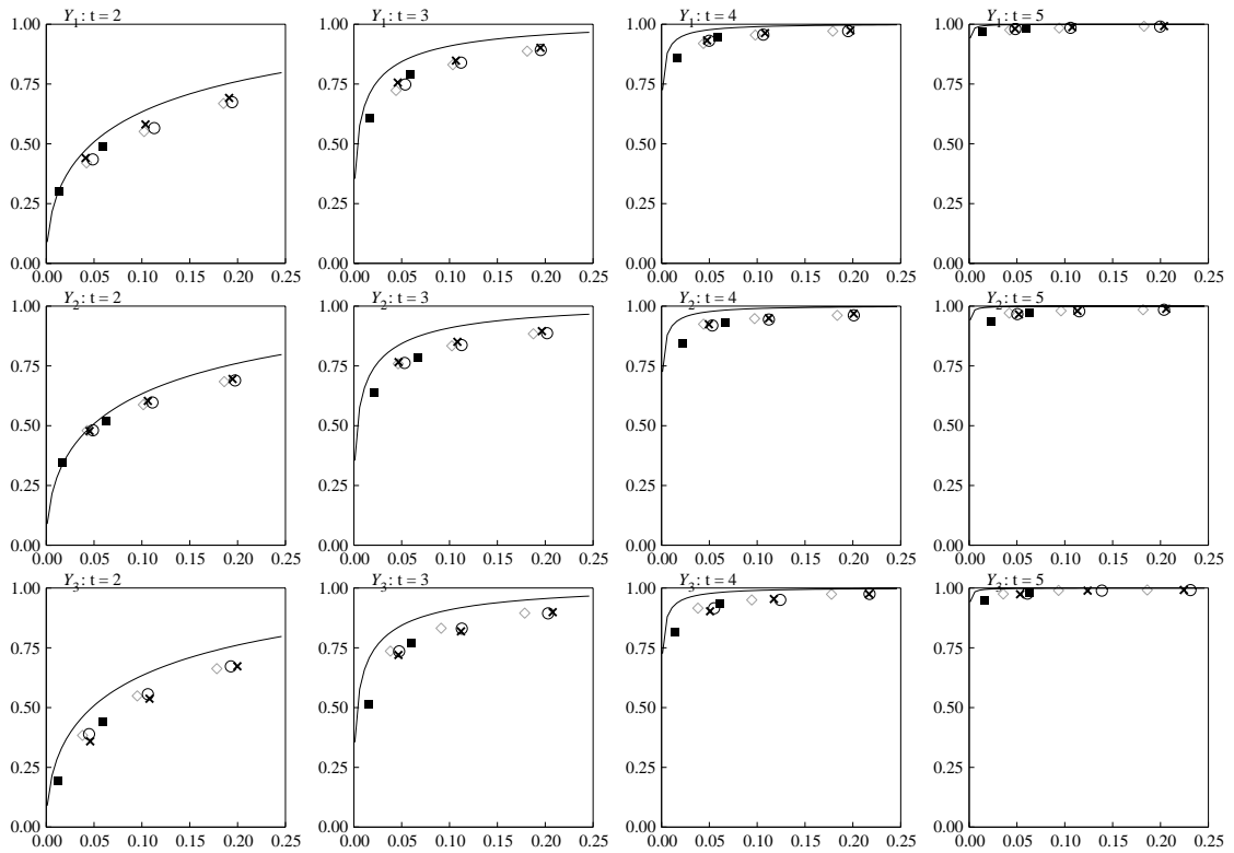
Figure 3: DGP (3.2): Power – size trade-off
