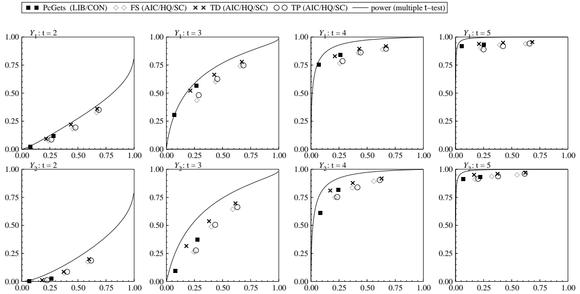
Figure 4: DGP (3.1): Selection versus non-deletion probabilities
