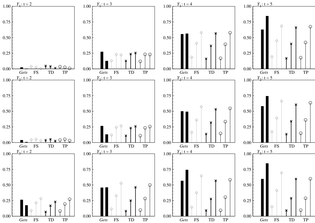
Figure 7: Probability of finding the DGP (3.2)
