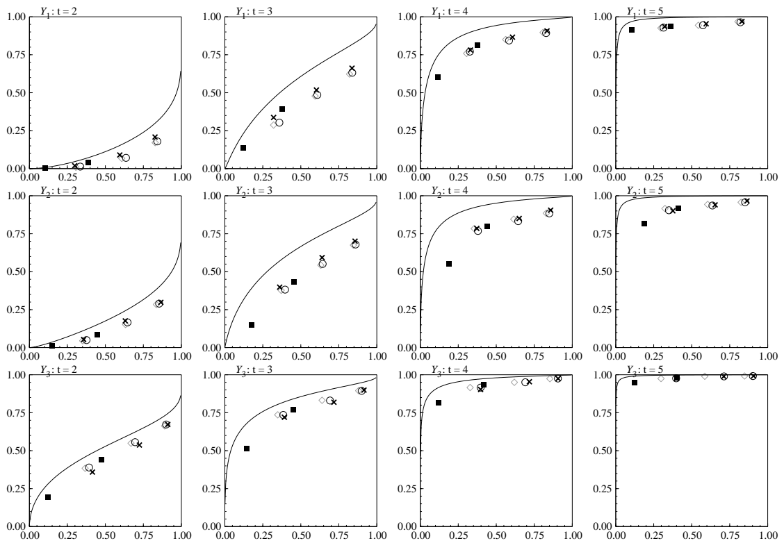
Figure 5: DGP (3.2): Selection versus non-deletion probabilities
