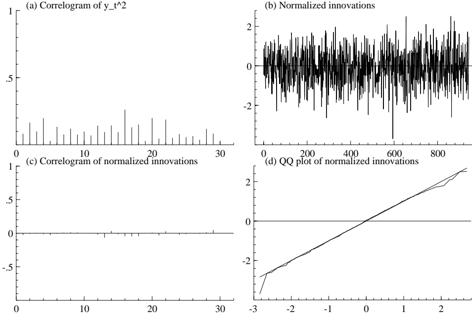
Figure 8: Diagnostic checks. Graph (a): correlogram of y_t^2 . Graph (b): normalised innovations. Graph (c): the corresponding correlogram. Graph (d): associated QQ-plot.
