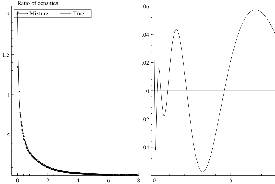
Figure 3: Mixture approximation to \chi_1^2 density. Left: \chi_1^2 density and mixture approximation. Right: the log of the ratio of the \chi_1^2 density to the mixture approximation.
