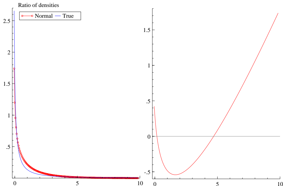
Figure 1: Log-Normal approximation to \chi_1^2 density. Left is the \chi_1^2 density and the log-normal approximation which is used in the quasi-likelihood approach. Right is the log of the ratio of the \chi_1^2 density to the approximation.
