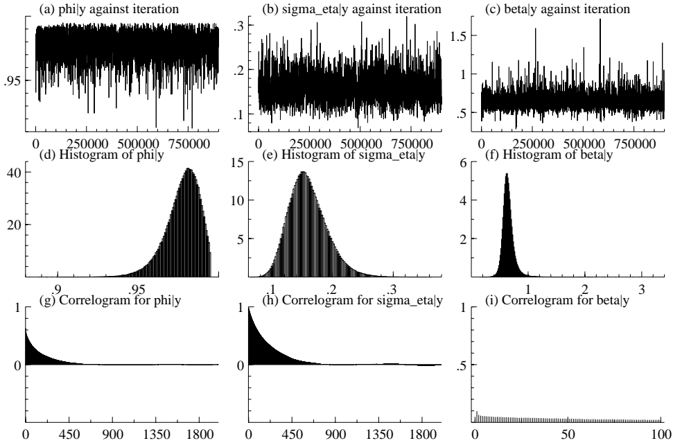
Figure 2: Single move Gibbs sampler for the Sterling series. Graphs (a)-(c): simulations against iteration. Graphs (d)-(f): histograms of marginal distribution. Graphs (g)-(i): corresponding correlograms for simulation. In total 1,000,000 iterations were drawn, discarding the first 50,000.
