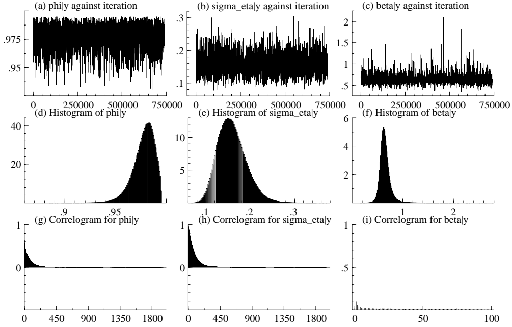
Figure 4: Mixture sampler for Sterling series. Graphs (a)-(c): simulations against iteration. Graphs (d)-(f): histograms of marginal distribution. Graphs (g)-(i): corresponding correlograms for simulation. In total 750,000 iterations were drawn, discarding the first 10,000.
