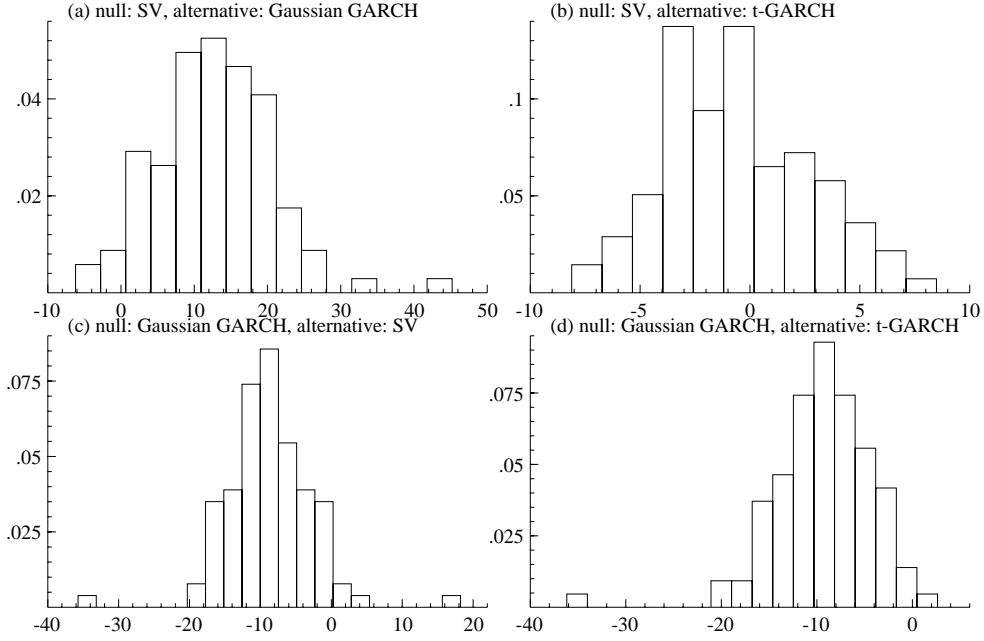
Figure 9: Non-nested testing. Graphs (a)-(b) LR_y computed when SV is true. Graph (a): SV against a GARCH model. Graph (b): SV against a t-GARCH. The observed values are 19.14 and -2.68 respectively, which are 80th and 29th out of the 100 samples. Graphs (c)-(d): LR_y computed when GARCH model is true. Graph (c): GARCH against SV. Graph (d): GARCH against t-GARCH. The observed values are 19.14 and -2.68 respectively, which ranks them 100th and 79th out of the 100 samples.
