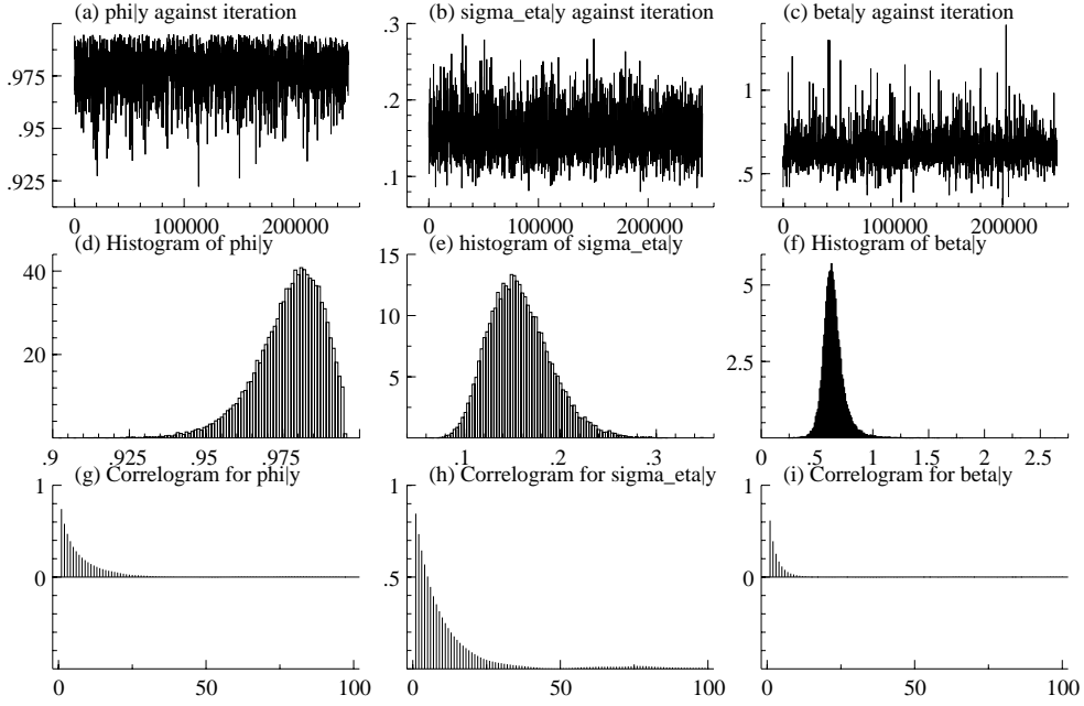
Figure 5: The integration sampler for Sterling series. Graphs (a)-(c): simulations against iteration. Graphs (d)-(f): histograms of marginal distribution. Graphs (g)-(i): corresponding correlograms for simulation. In total 250,000 iterations were drawn, discarding the first 250.
