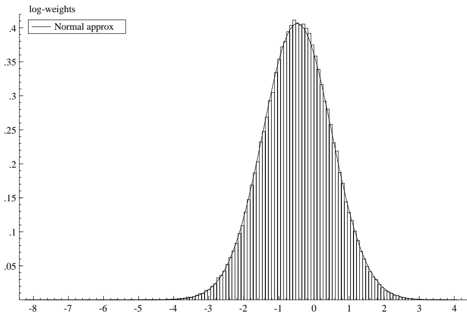
Figure 6: Histogram of the log of the M \times c^j for 250,000 sweeps for the integration sampler and a corresponding approximating normal density with fitted mean and standard deviation. All the weights around zero would indicate a perfect sampler.
