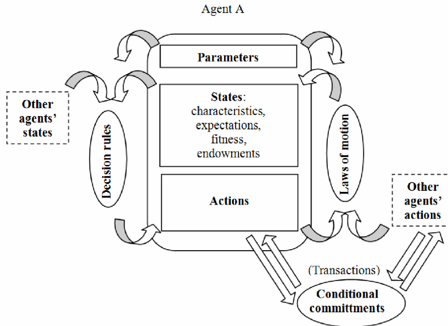
Figure 2: Scheme of an economic agent.
